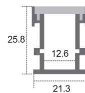
CL-Alu-5020-BL (With Black and White PC Cover)
