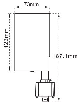
20 Watt Track Light
