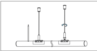
CL-ST-NEON25-360D-Horizontal lifting kit PC tube length: 38mm Length of wire rope: 2m
