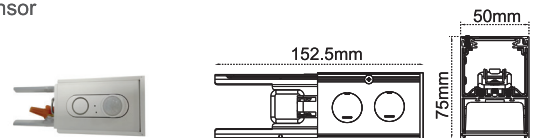
CL-LL1A-PSMI-PRO Plug in sensor
