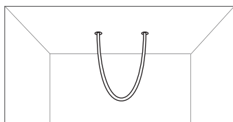
CL-ST-NEON25-360D-Embedded kit with trim Size: \Phi 64 \times H20 \text{ mm} Mounting hole size: \Phi 40\text{mm}
