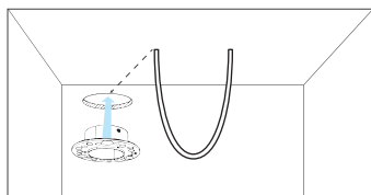
CL-ST-NEON25-360D-Embedded kit trimless Size: \Phi 64 \times H20\text{mm} Mounting hole size: \Phi 40\text{mm}
