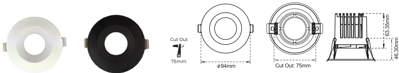
CL-DL3-3R Round Frame with Trim
