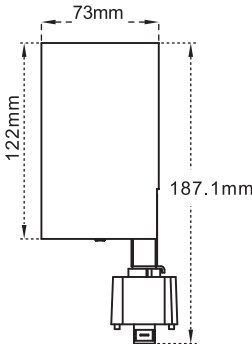
20 Watt Track Light
