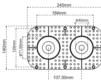
Trim-less Double Round Frame
