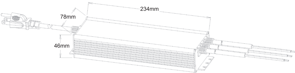
192W Dimensions: 258x78x46 mm(LxWxH) The overall length including the end caps
