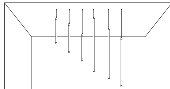
CL-ST-NEON25-360D-single end vertical surface mount kit B
