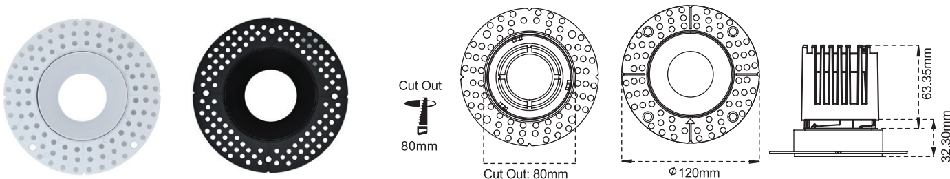
CL-DL3-3RT Trim-less Round Frame
