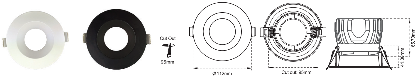
CL-DL3-3.5R Round Frame with Trim
