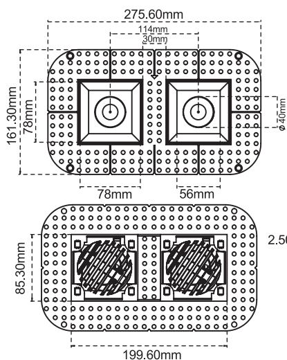
Trim-less Double Square Frame
