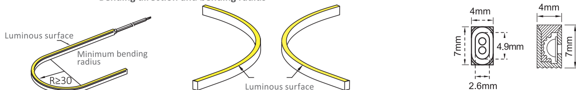
Bending direction and bending radius
