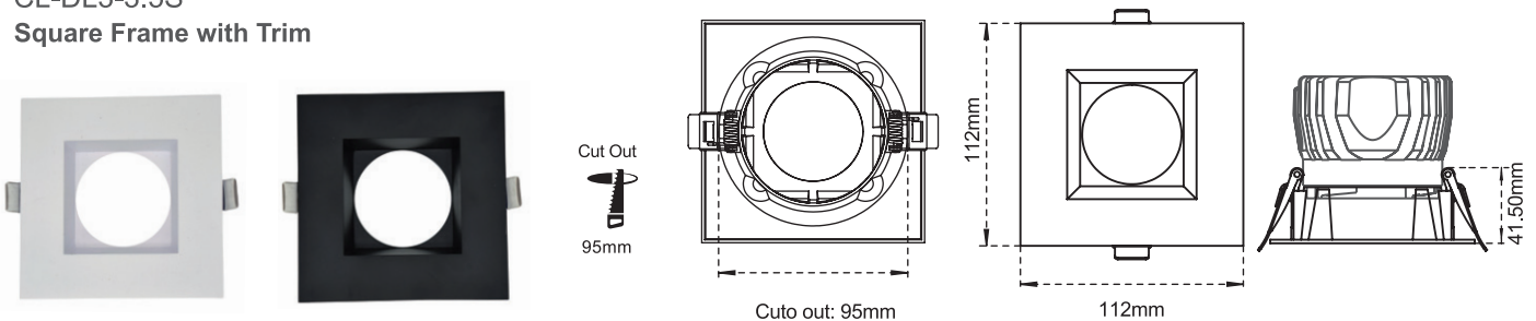
CL-DL3-3.5ST Trim-less Square Frame
