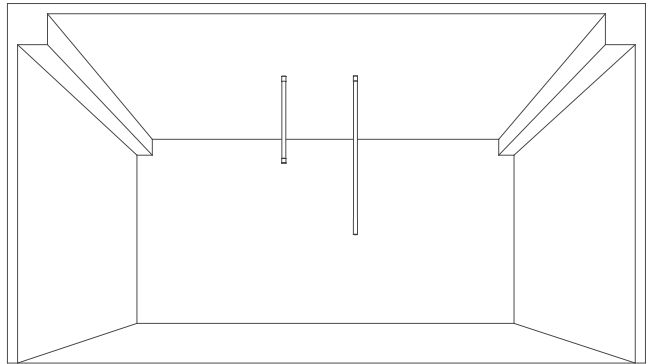
CL-ST-NEON25-360D-single end vertical surface mount kit B
