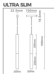
CL-Pendant35-R-A-20-ULS
