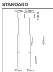
CL-Pendant35-R-A-20
