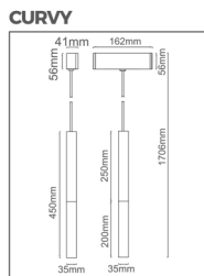
CL-Pendant35-R-A-20-D9
