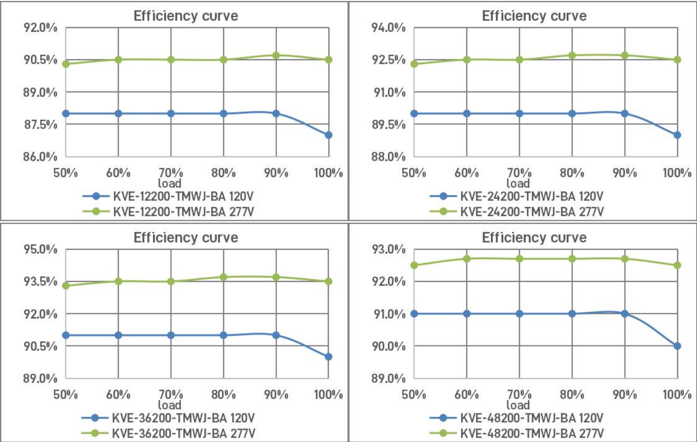
Efficiency Curve (efficiency vs output load)
