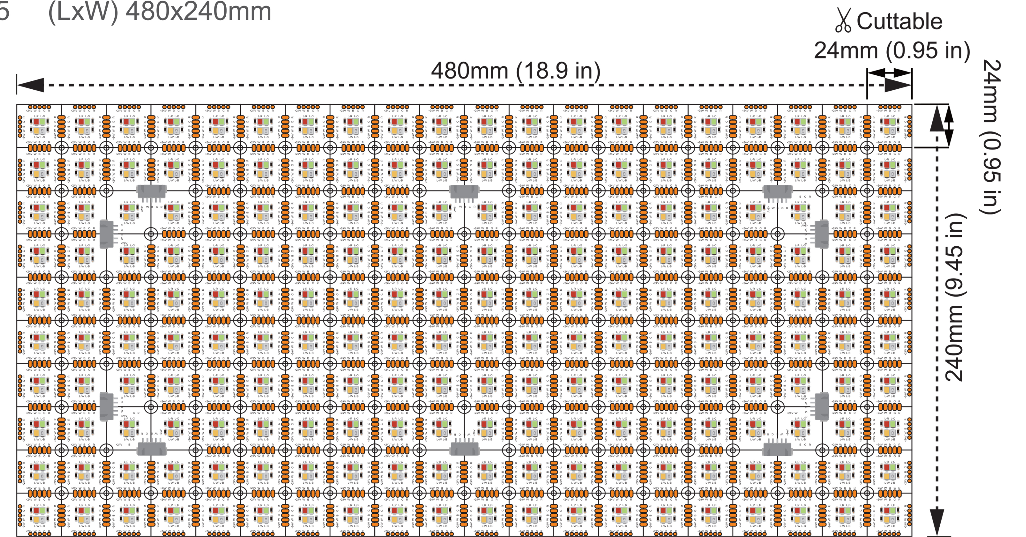
CL-LSH-5P-BBW Double head connector with 6cm/30cm wire, 20Awg, 5-pin
