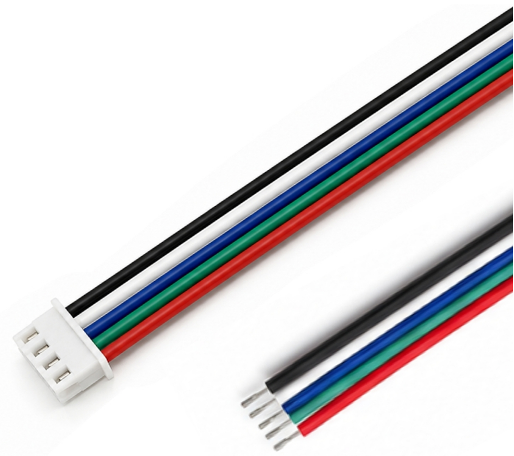
CL-LSH-5P-XBW30 Single head connector with 30cm wire, 20Awg, 5-pin
