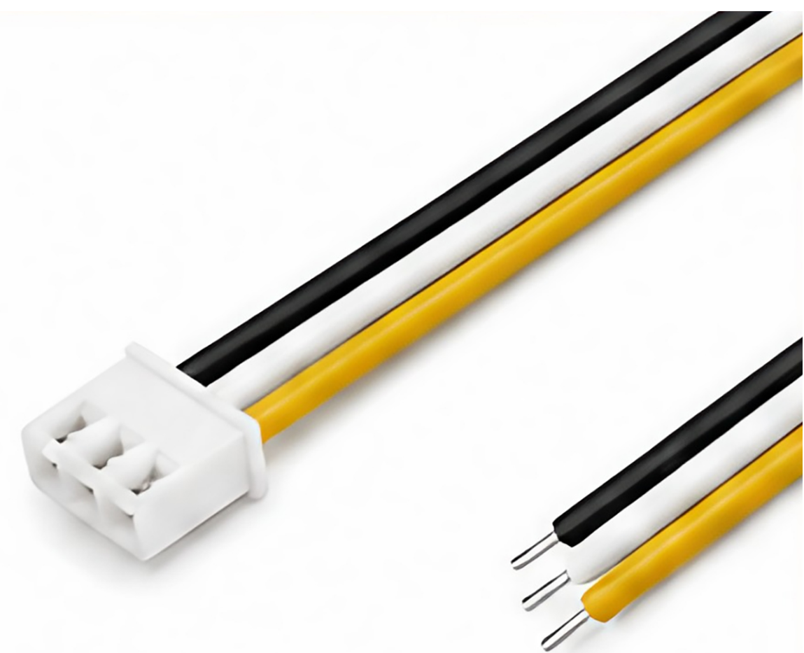
CL-LSH-3P-XBW30 Single head connector with 30cm wire, 20Awg, 3-pin
