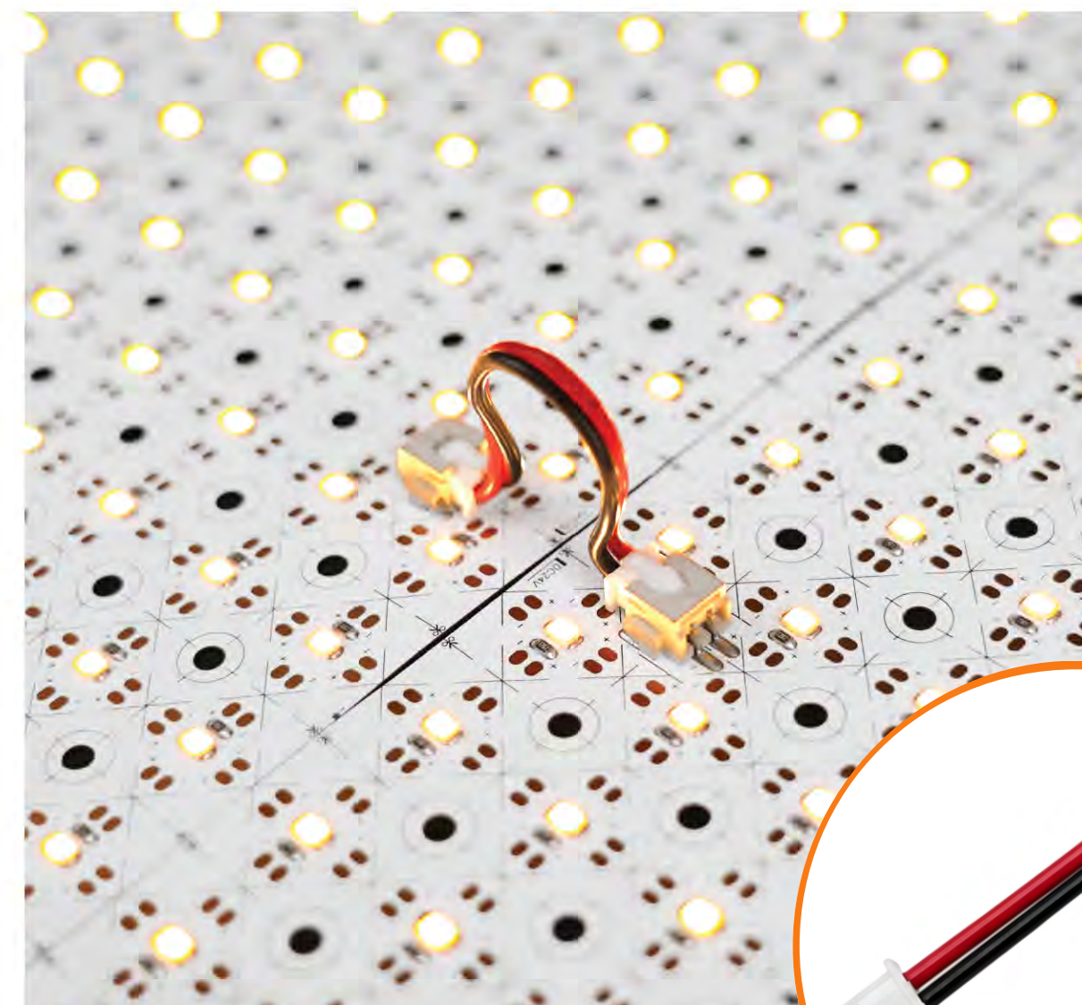
CL-LSH-2P-BBW Double head connector with 6cm/30cm wire, 20Awg, 2-pin
