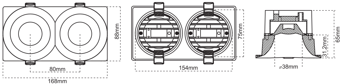
CL-DL6-D18-5CCT Cut out: 141x75mm
