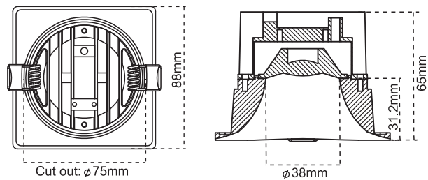
CL-DL6-S9-5CCT Cut out: 76mm
