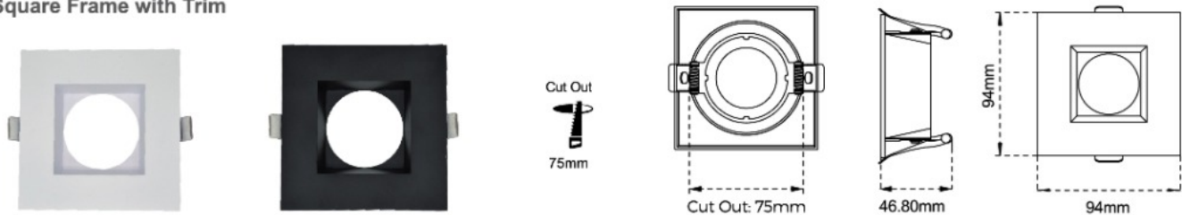
CL-DL3-3S Square Frame with Trim
