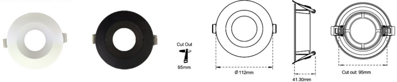
CL-DL3-3.5R Round Frame with Trim
