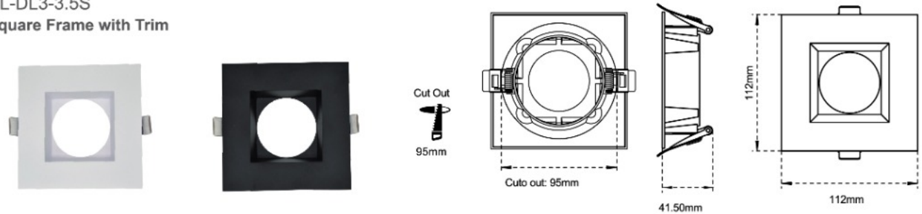
CL-DL3-3.5ST Trim-less Square Frame
