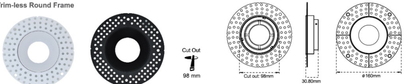
CL-DL3-3.5RT Trim-less Round Frame
