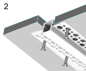
Drywall Linear Aluminum LED Channel
